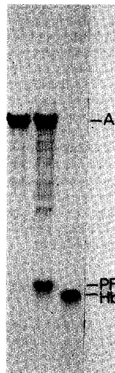
Fig. 3. 7.5% polyacrylamide–sodium dodecyl sulphate slab gel, Tris–bicine buffer system of (left) platelet actin, (centre) platelet profilactin, (right) haemoglobin marker.
