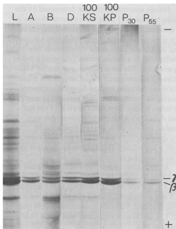
Fig.2. Isoelectric focussing in tube gels of platelet subfractions. \beta , \gamma are actin subforms. 'L', cell lysate; 'A', soluble fraction; 'B', membranes; 'D', pellet; 100 KS, 100 KP supernatant and pellet, respectively, from 100\,000 \times g centrifugation of 'A'; P 30 , partially purified actin, 0–30% ammonium sulphate fraction, i.e., contains only uncomplexed actin; P 55 , 30–55% ammonium sulphate fraction, i.e., profilactin.
